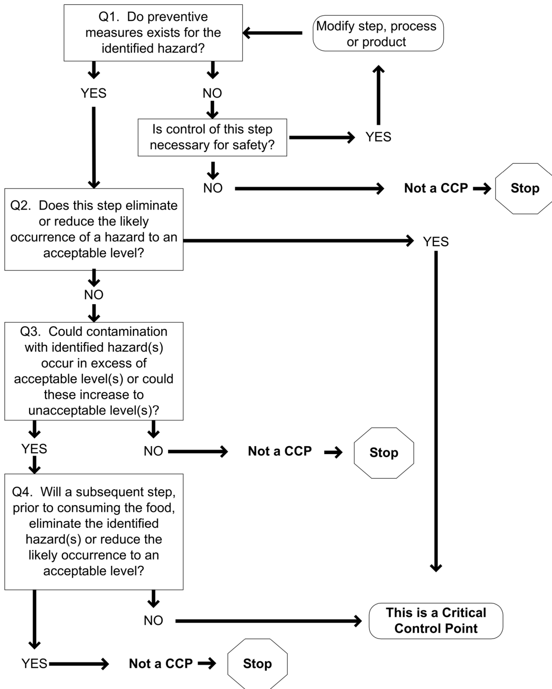
Figure 2: CCP Decision Tree (Stevenson and Bernard, 1995)
